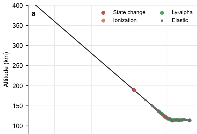
Single H^+ trajectory, 400 km/s, atmospheric segment
