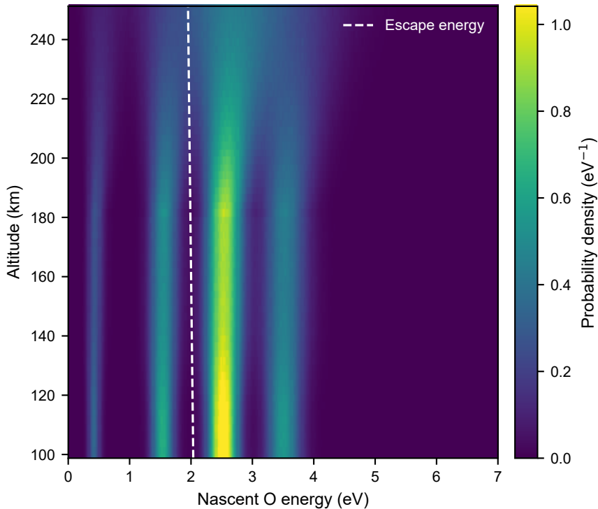
Nascent hot O energy probability density, L_s = 0^\circ , F070
