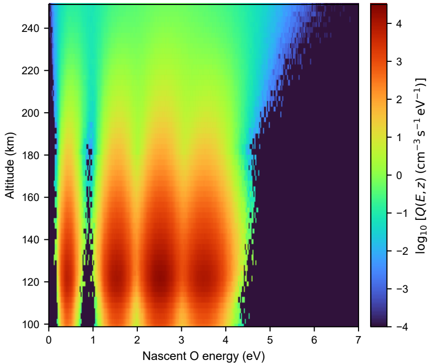
Hot O spectral production rate, L_S = 0^\circ , F070
