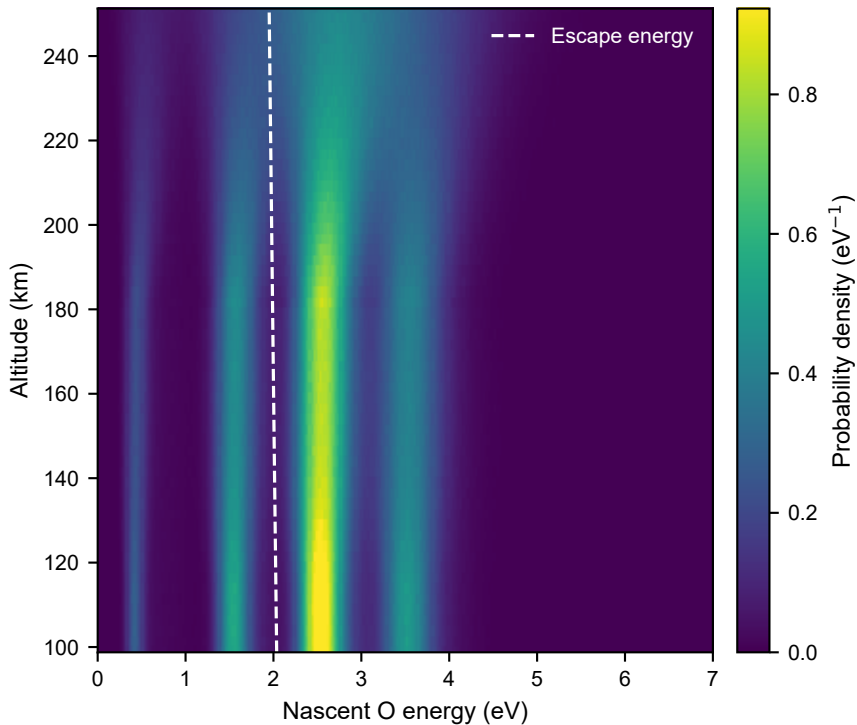
Nascent hot O probability with \text{O}_2^+ vibration, L_s = 0^\circ , F070
