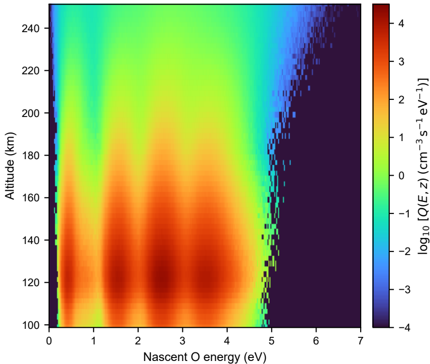
Hot O production with \text{O}_2^+ vibration, L_S = 0^\circ , F070
