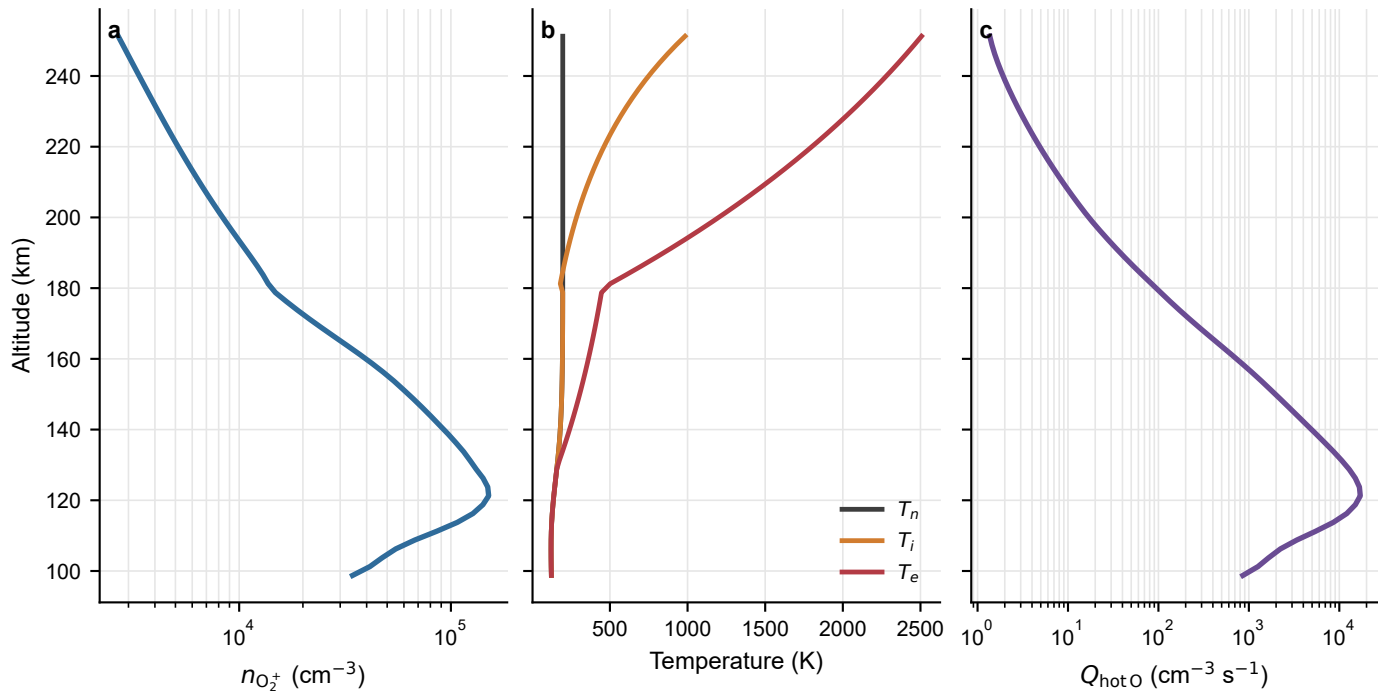
MGITM baseline profiles, L_s = 0^\circ , F070 Nearest subsolar grid columns: lon = 27.5^\circ , lat = -2.5, 2.5^\circ , SZA = 2.73^\circ
