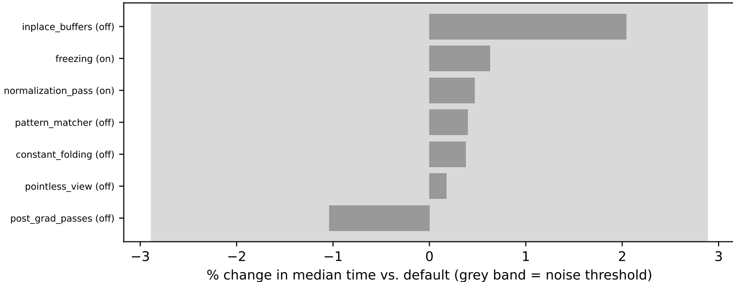
gpt2_prefill: toggling one switch at a time (Chideras-MacBook-Pro-2)
