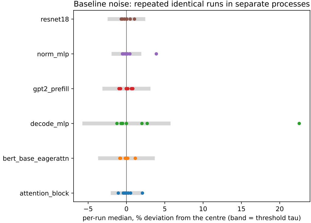
Figure 1: Per-run medians of identical baseline runs, as deviation from the centre; the grey band is \tau .
