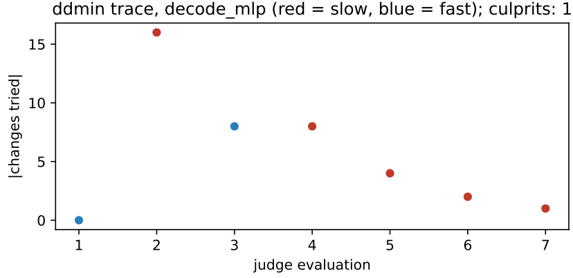
Figure 3: ddmin search trace for decode_mlp: each point is one judge evaluation.
