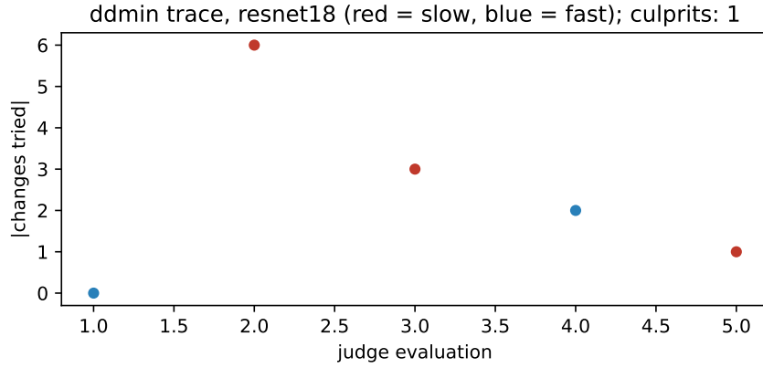
Figure 5: ddmin search trace for resnet18: each point is one judge evaluation.
