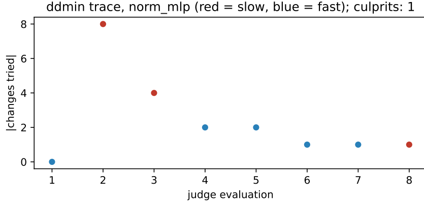
Figure 4: ddmin search trace for norm_mlp: each point is one judge evaluation.
