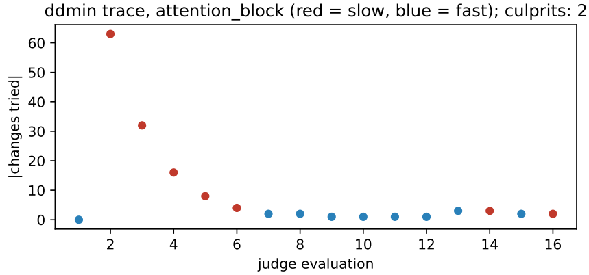
Figure 6: ddmin search trace for attention_block: each point is one judge evaluation.
