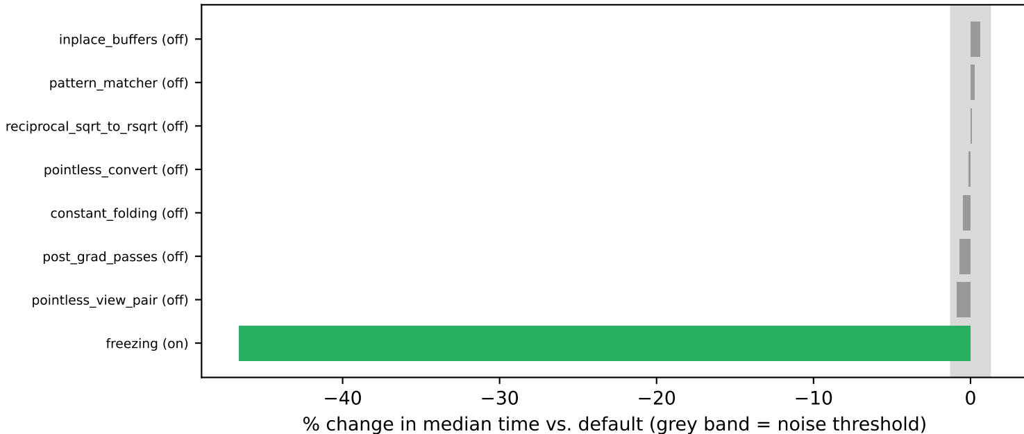
norm_mlp: toggling one switch at a time (VM Xeon)
