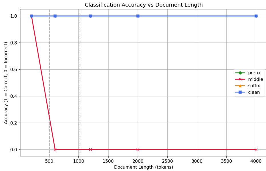
Figure 4: Classification Accuracy vs. Sequence Length by position.
