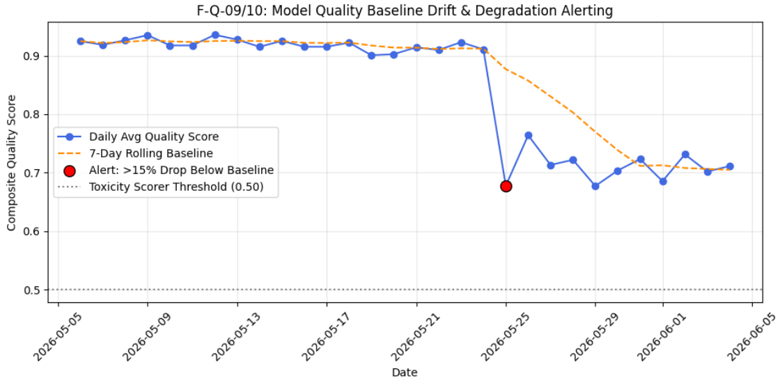
Figure 1: Model Quality Baseline Drift and Degradation Alerting Plot.
