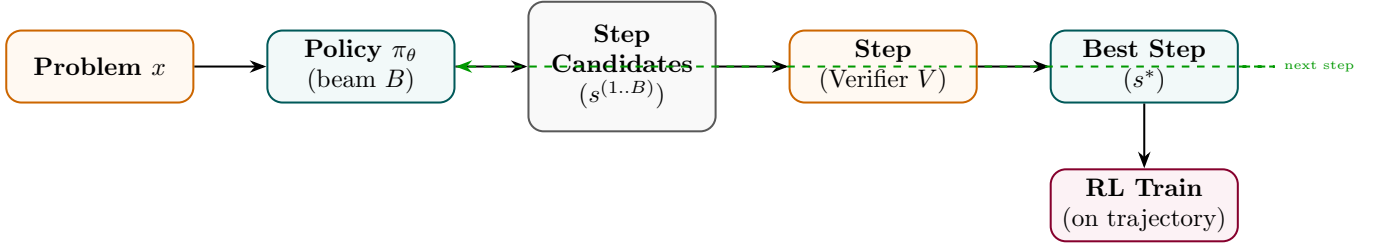
Figure 38: Search-RL: at each step, beam search generates candidates; verifier selects best; policy trained on trajectory.
