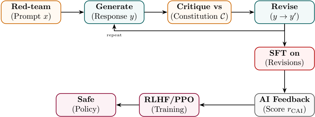
Figure 11: Constitutional AI: critique-revise loop creates SFT data; AI feedback from constitution guides RLHF.
