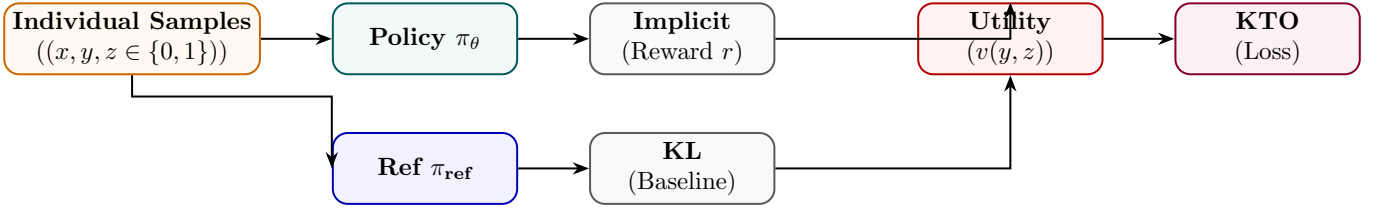
Figure 5: KTO: each sample is individually labelled good/bad; utility function uses prospect theory asymmetry.
