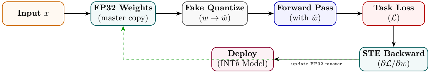
Figure 17: QAT: fake quantization in forward pass; STE allows gradients to flow to FP32 master weights.
