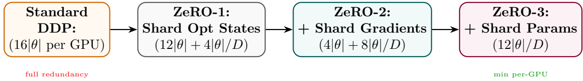
Figure 32: DeepSpeed ZeRO stages: each stage shards an additional component, progressively reducing per-GPU memory.
