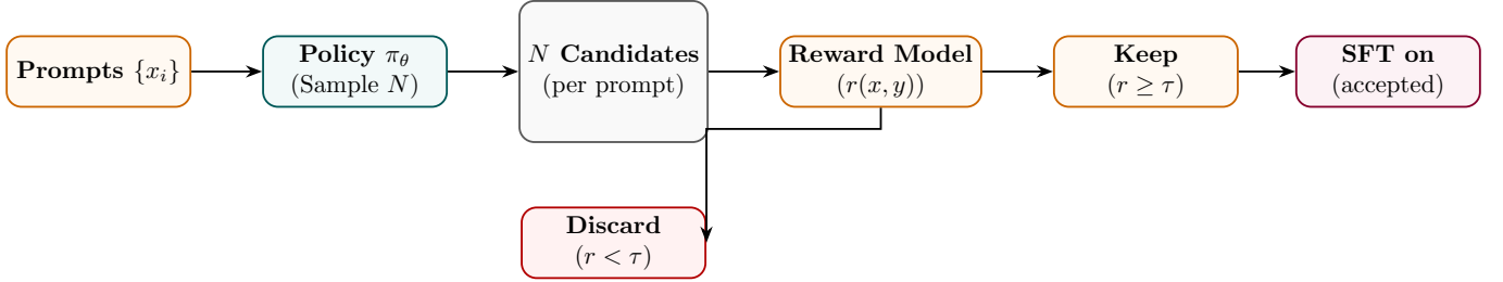
Figure 5: Rejection Sampling: N completions generated; only those above reward threshold kept for SFT.
