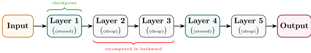
Figure 29: Gradient Checkpointing: only checkpoint activations stored; intermediate activations recomputed in backward.
