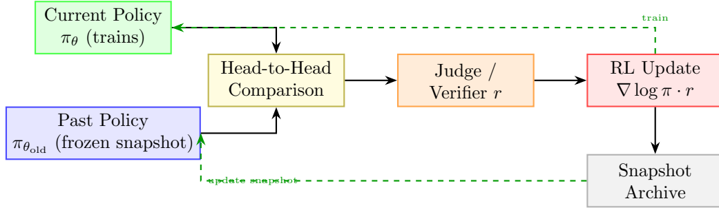
Figure 17: Self-Play RL: current policy competes against a frozen past snapshot; win/loss drives RL updates.
