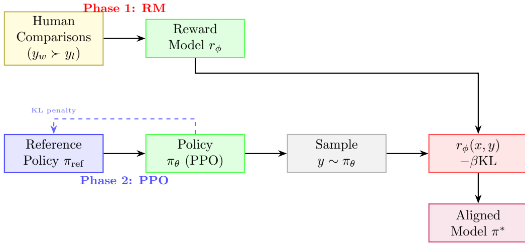
Figure 1: RLHF: reward model trained on human comparisons then used to guide PPO policy optimisation.
