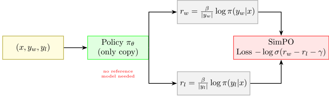
Figure 6: SimPO: length-normalised log-probs replace the reference log-ratio; margin \gamma enforces quality gap.
