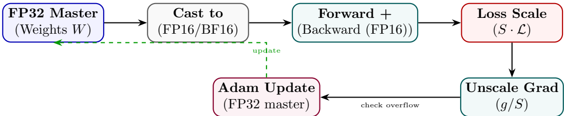
Figure 73: Mixed Precision Training: FP16 compute with FP32 master weights; loss scaling prevents gradient underflow.
