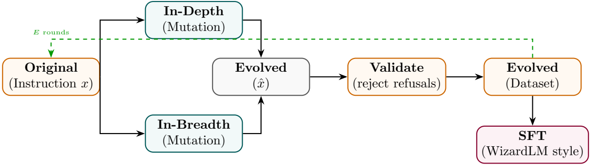
Figure 47: Evol-Instruct: in-depth and in-breadth mutations generate harder variants; validated pool used for SFT.
