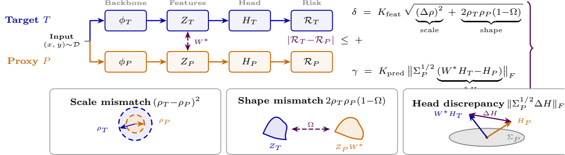
Figure 1: PRISM decomposition of the risk gap. The cross-entropy risk gap |\mathcal{R}_T - \mathcal{R}_P| between target T and proxy P is bounded by a feature alignment error \delta and a head discrepancy \gamma (Thm. ??). Under Procrustes alignment W^* = \arg \min_{W \in \mathcal{O}(d)} \|Z_T - Z_P W\|_F , \delta decomposes exactly into scale mismatch (\Delta\rho)^2 = (\rho_T - \rho_P)^2 and shape mismatch 2\rho_T\rho_P(1-\Omega)
