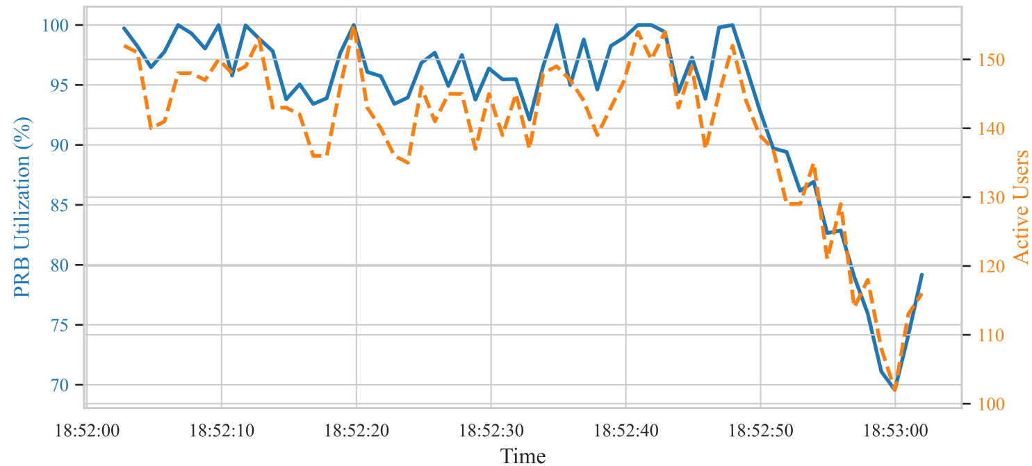
6G RAN Telemetry: Traffic Dynamics
