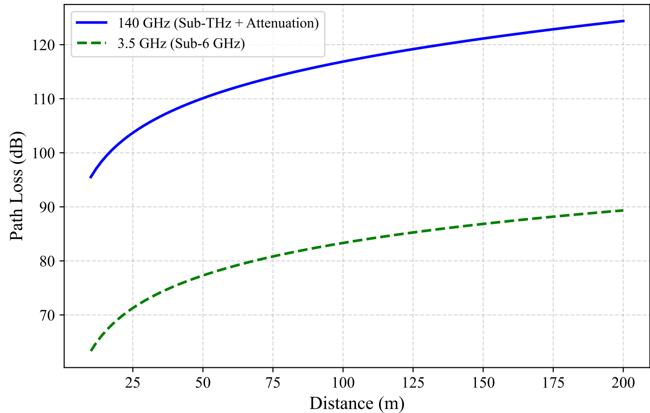
Theoretical Path Loss: Sub-6 GHz vs 140 GHz
