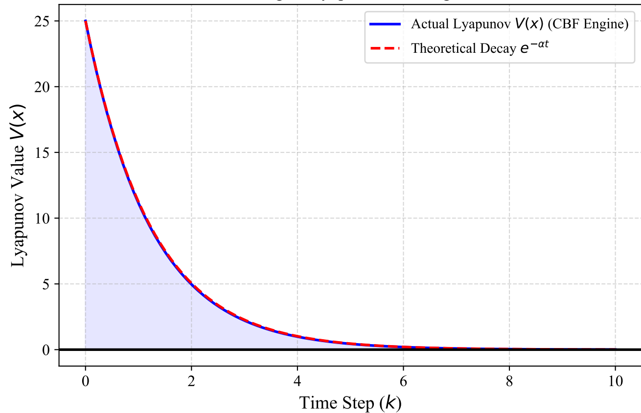
CBF Engine Lyapunov Convergence
