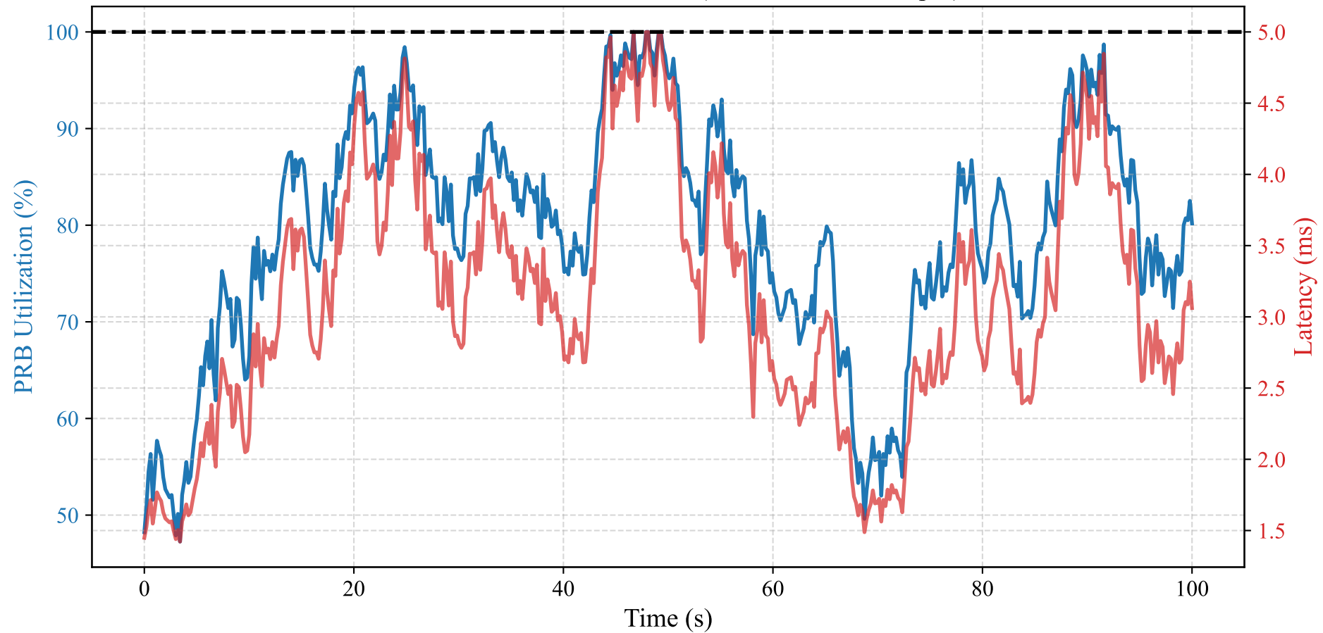
True Network State Evolution (RAN Simulator Output)
