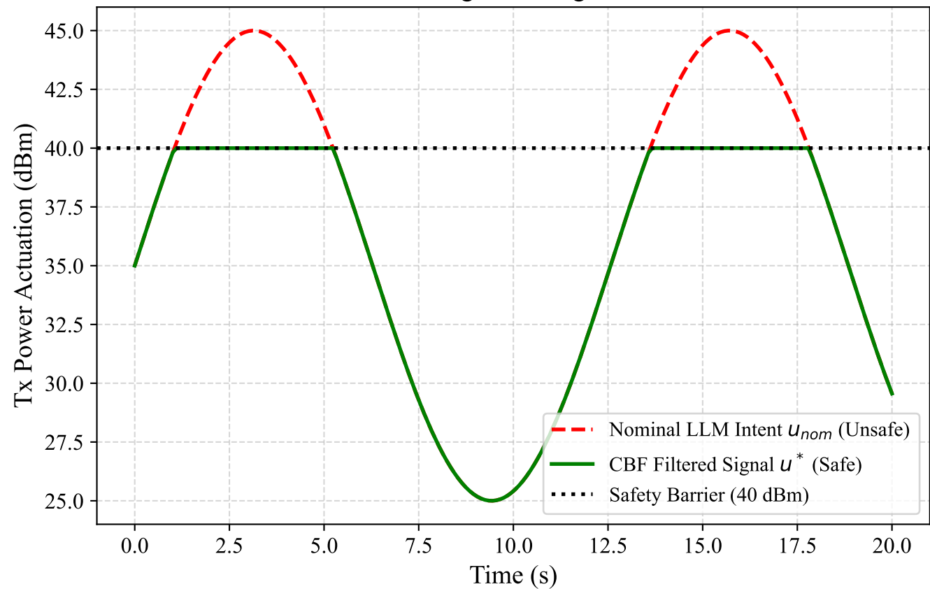
Actuation Filtering: CBF Engine Intervention
