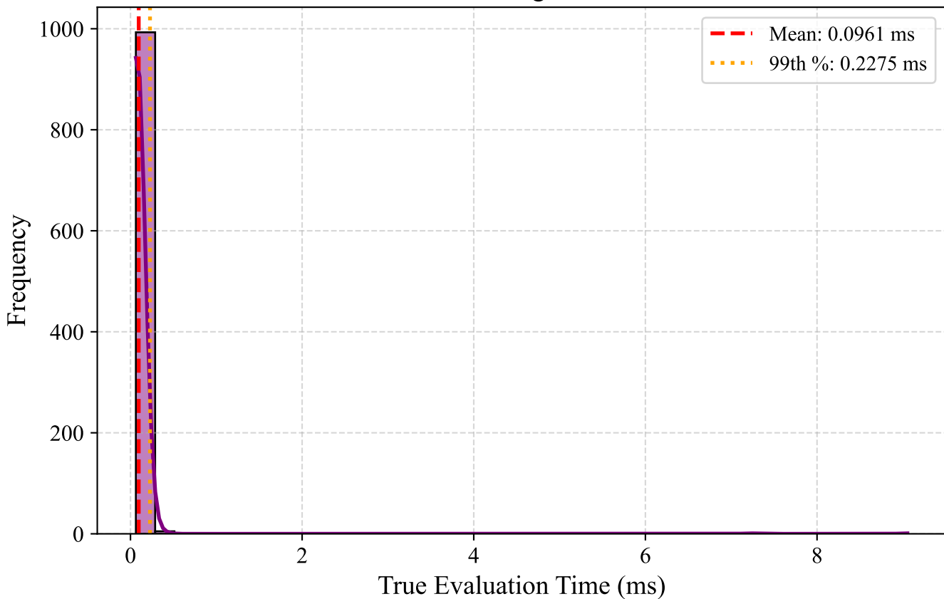
Distribution of CBF Engine Evaluation Time
