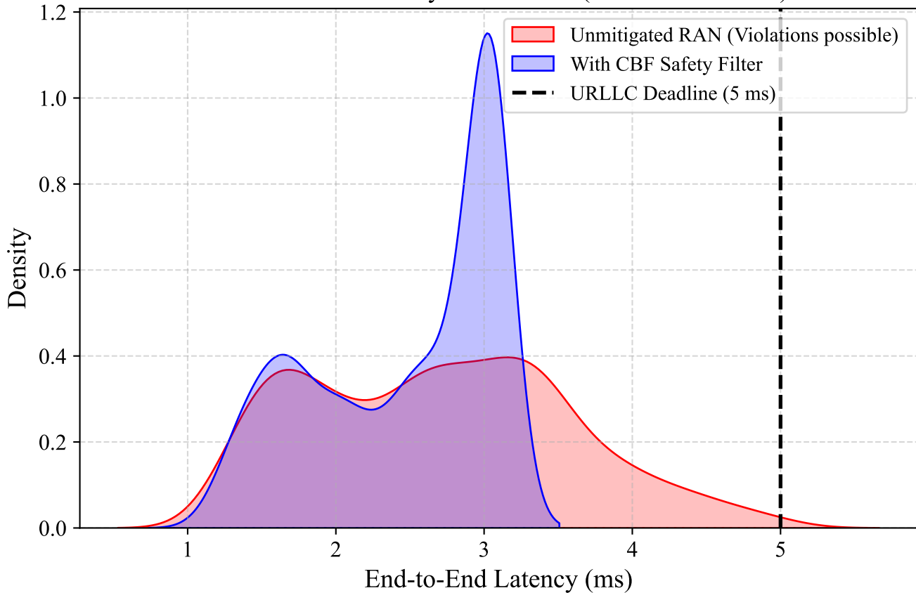
True URLLC Latency Distribution (O-U Process Data)
