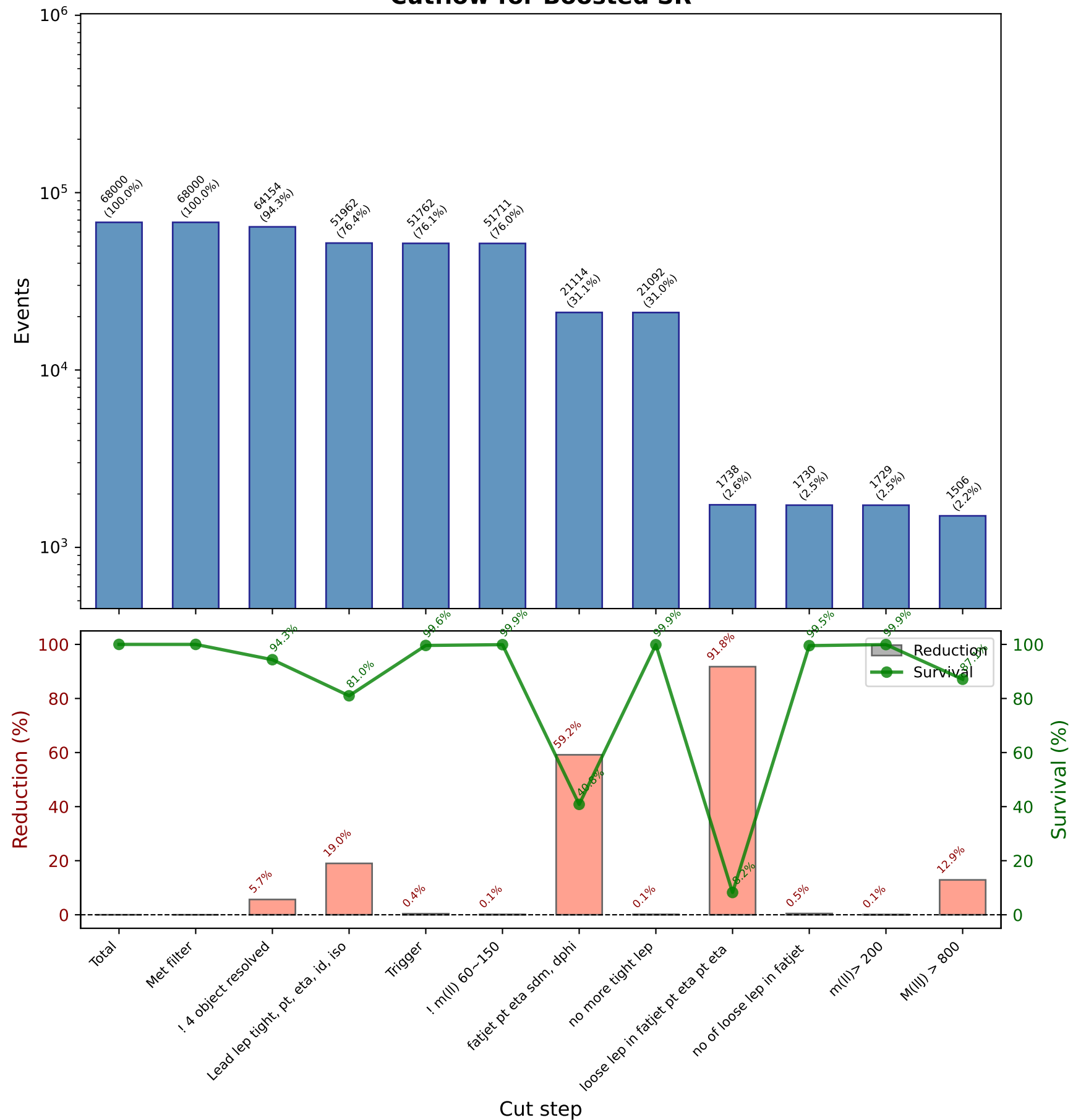
Cutflow for Boosted SR
