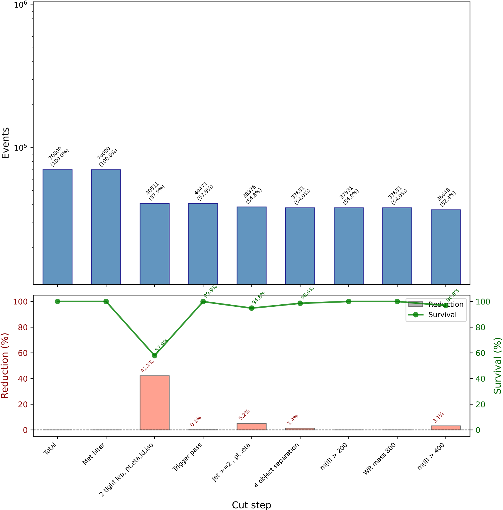
Cutflow for Resolved SR
