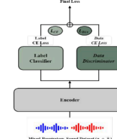
Figure 2: Overview of Adversarial fine-tuning with synthetic and real samples.
