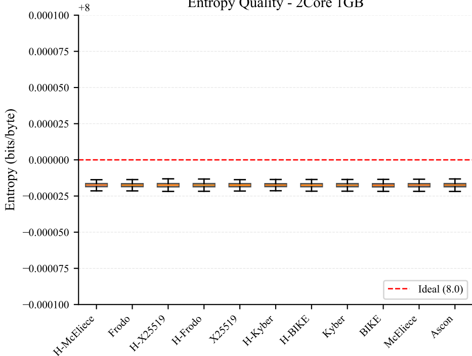
Entropy Quality - 2Core 1GB
