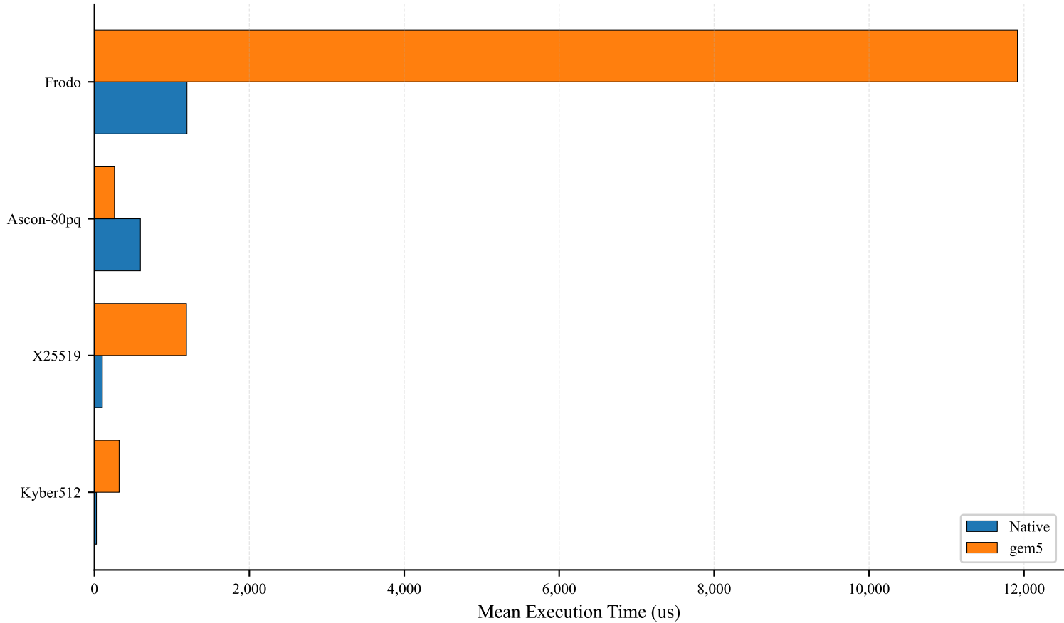
Native vs gem5 Mean Execution Time - 2Core 1GB
