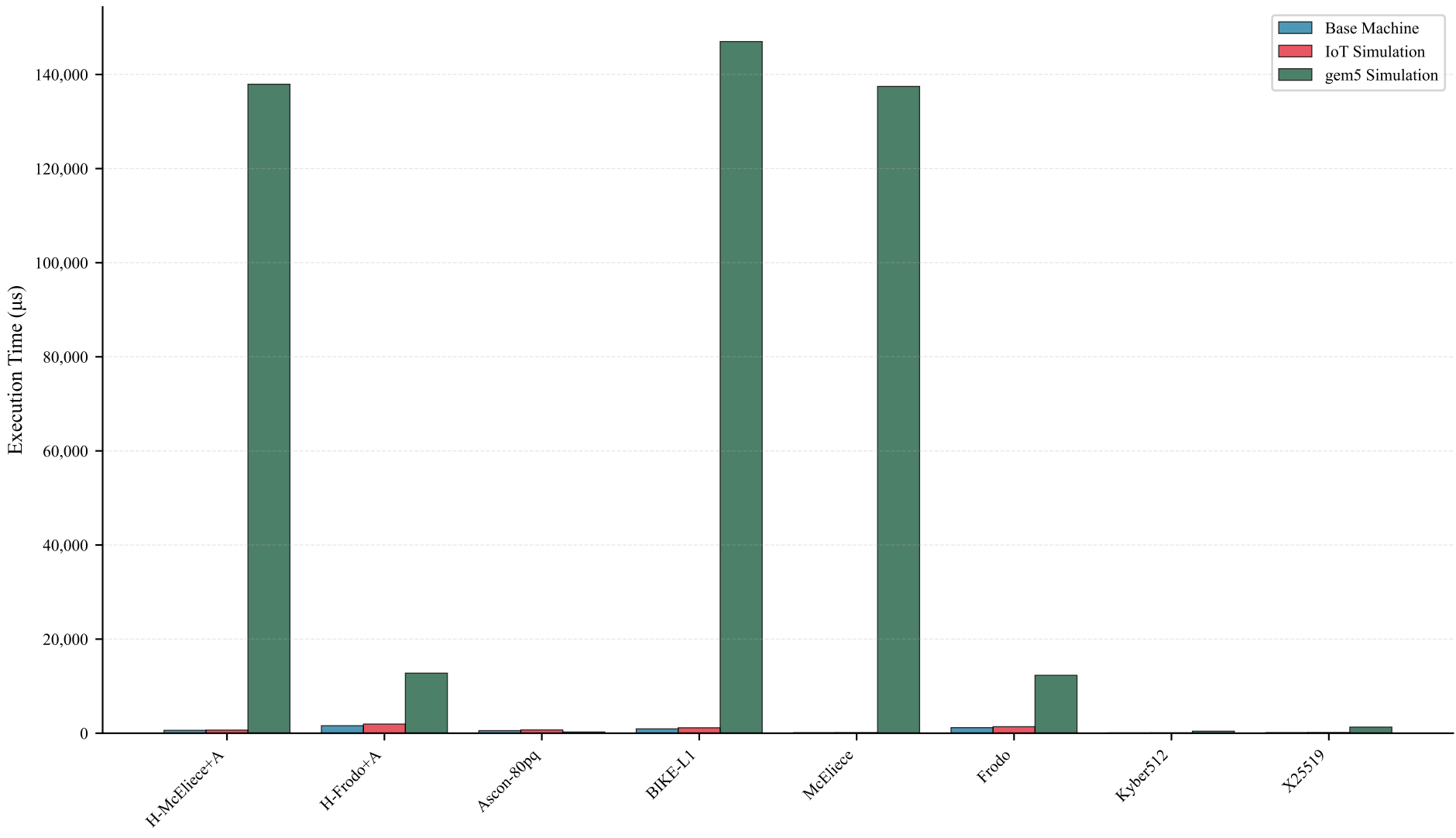
Performance Comparison Across Environments
