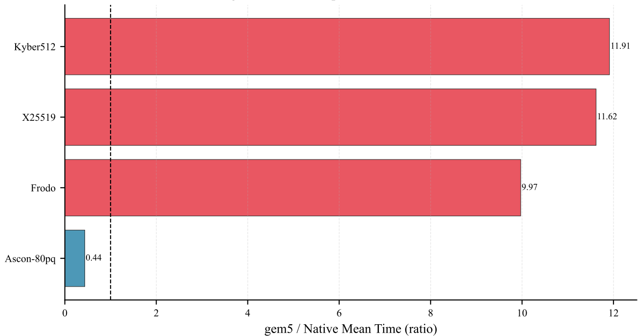
gem5 vs Native Speed Ratio - 2Core 1GB
