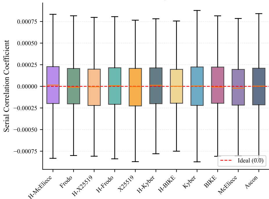
Randomness Quality - 2Core 1GB
