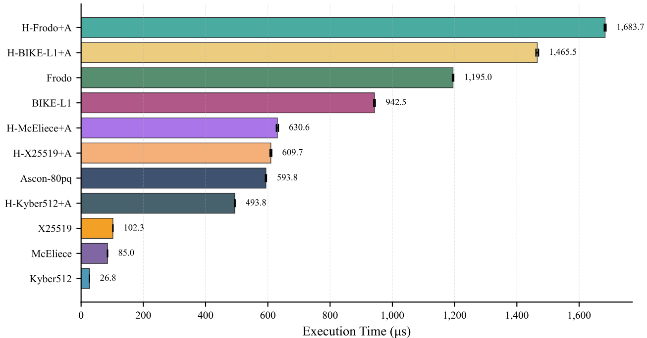
Mean Execution Time - 2Core 1GB Configuration
