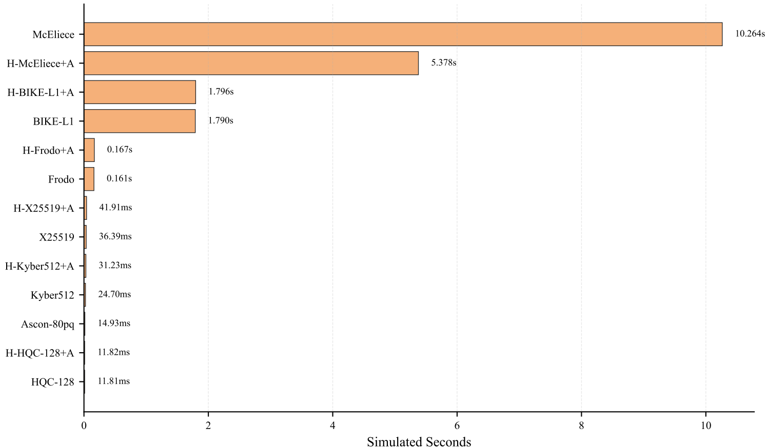
gem5 Simulation: Simulated Time
