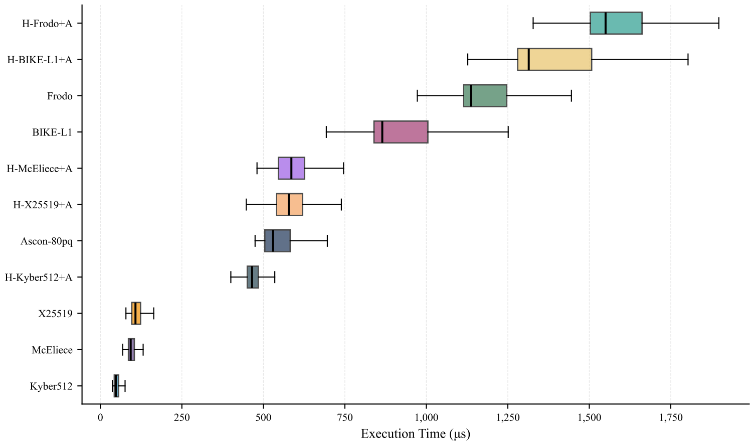
Execution Time Distribution
