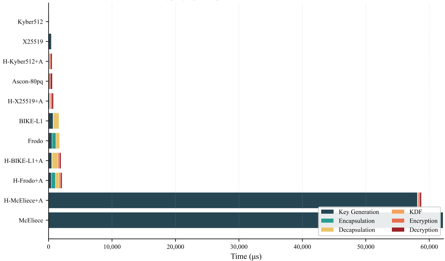
Cryptographic Operation Breakdown - 2Core 1GB
