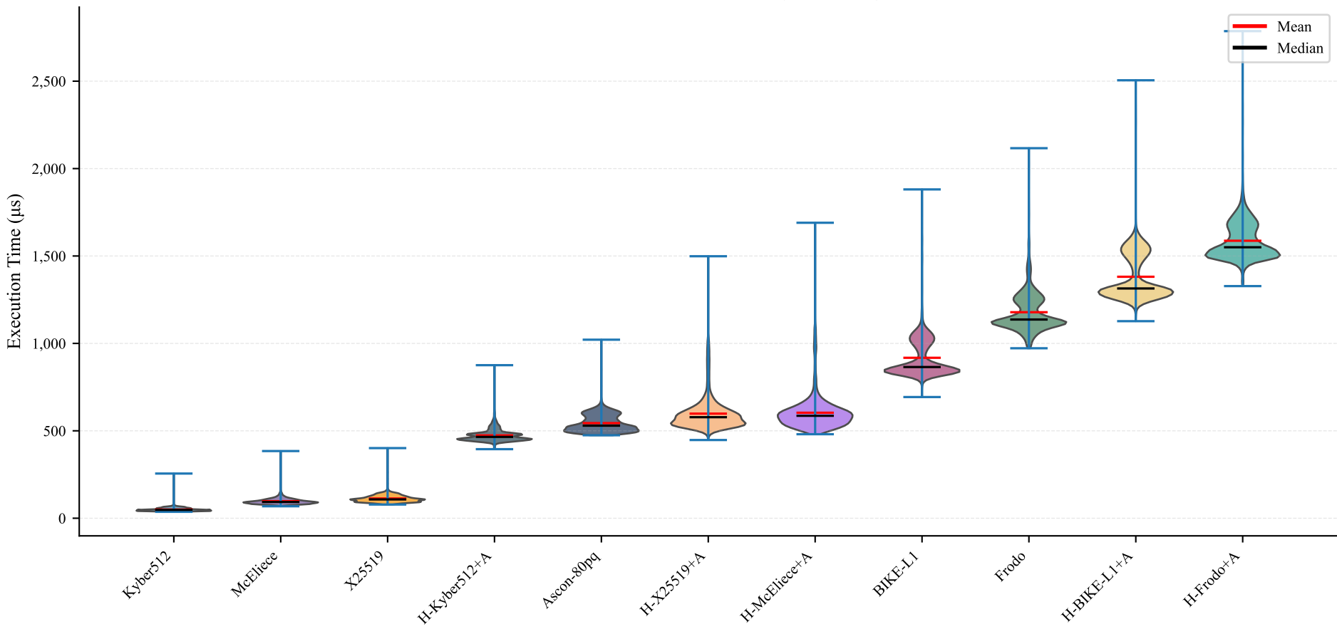
Execution Time Distribution (Violin Plot)
