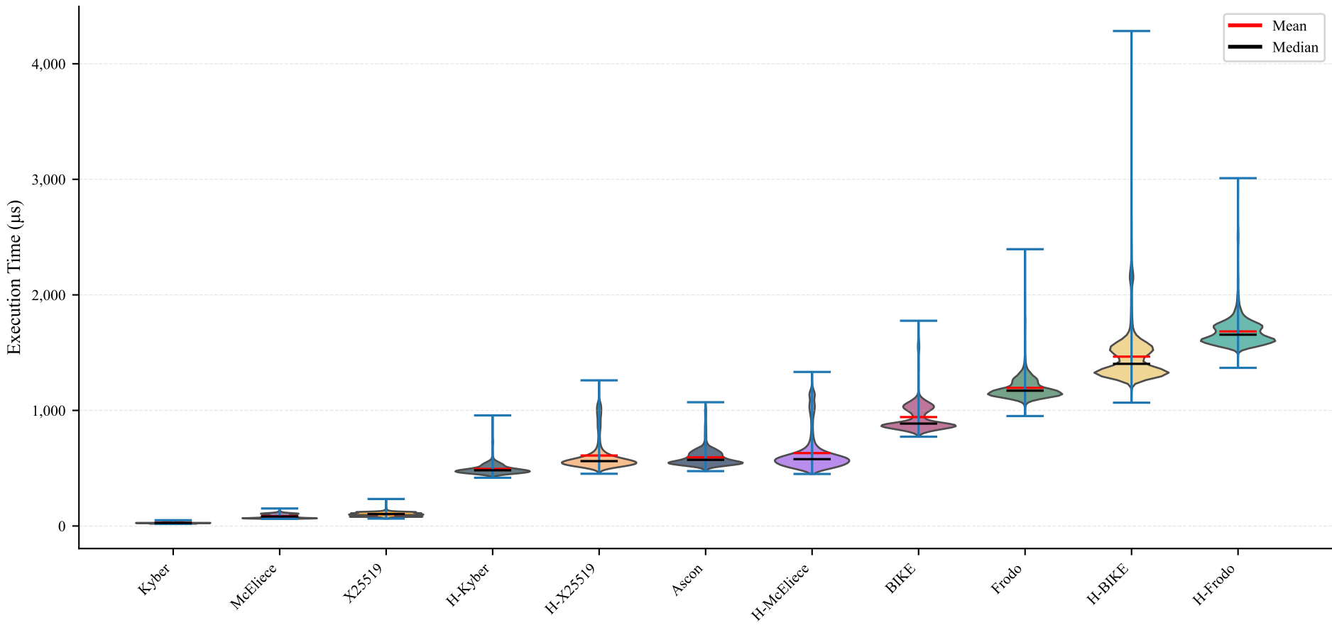
Execution Time Distribution (Violin Plot) - 2Core 1GB
