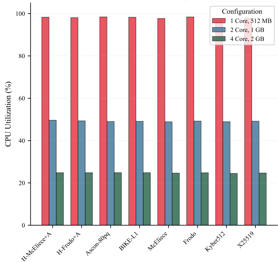
CPU Utilization by Configuration
