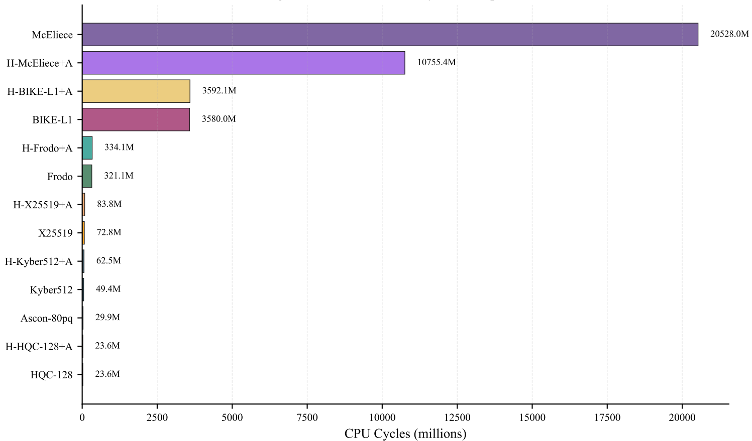
gem5 Simulation: CPU Cycles Comparison
