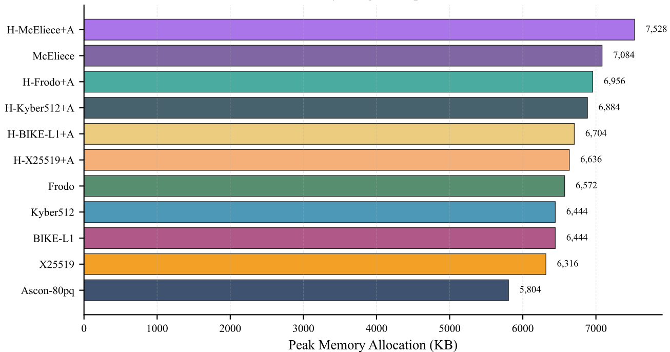
Memory Usage Comparison
