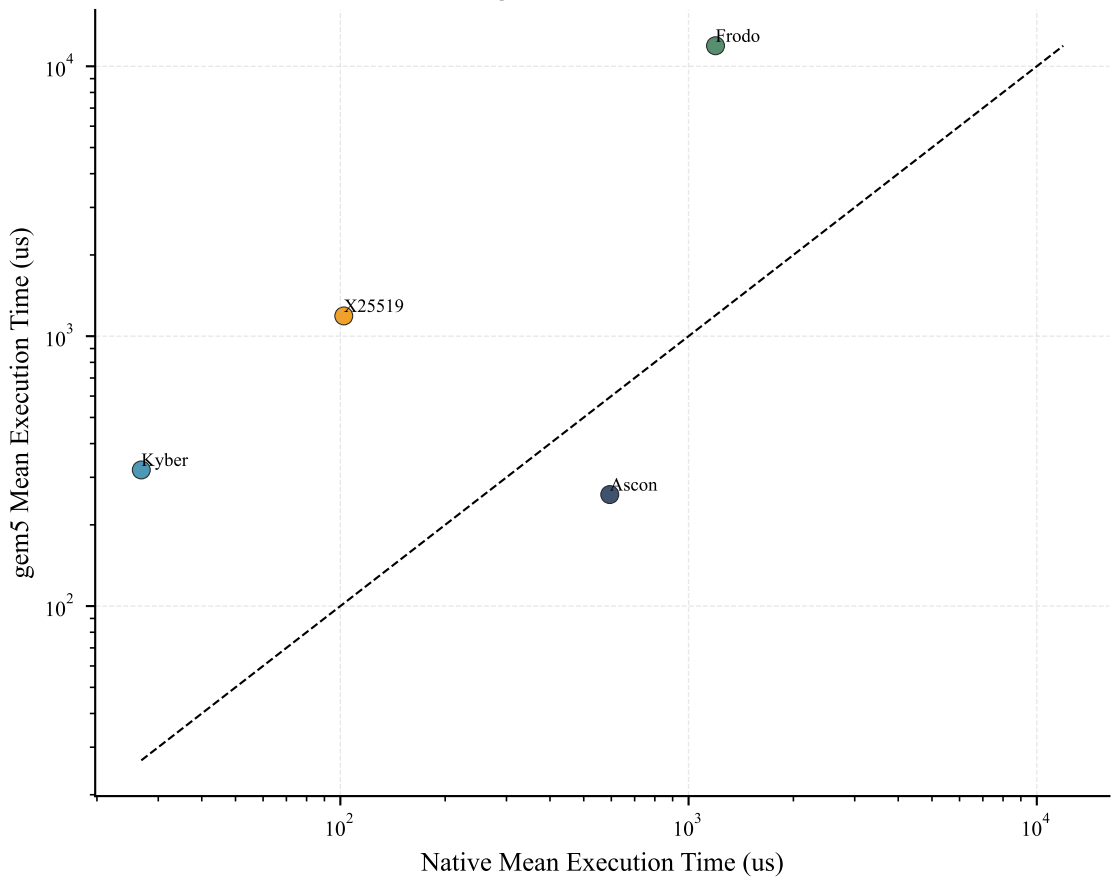
Native vs gem5 Mean Execution Time
