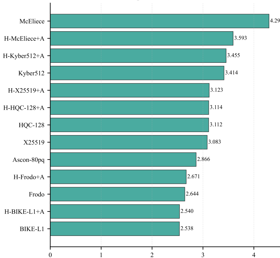
CPI Comparison (Lower = Better)
