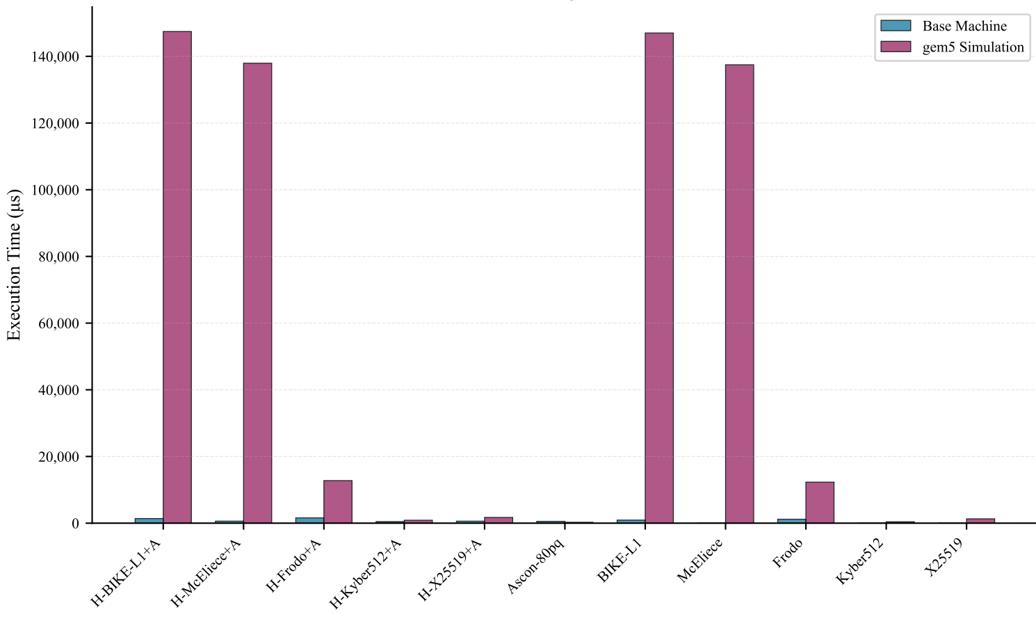
Base Machine vs gem5 Simulation
