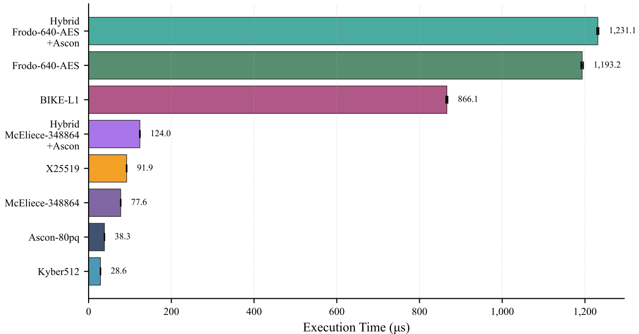
Mean Execution Time Comparison (Base Machine)
