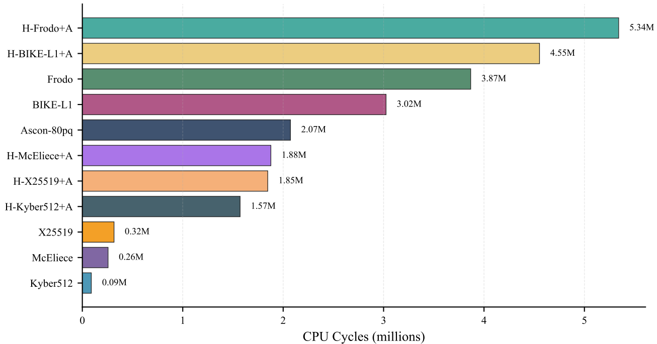
CPU Cycle Count Comparison - 2Core 1GB
