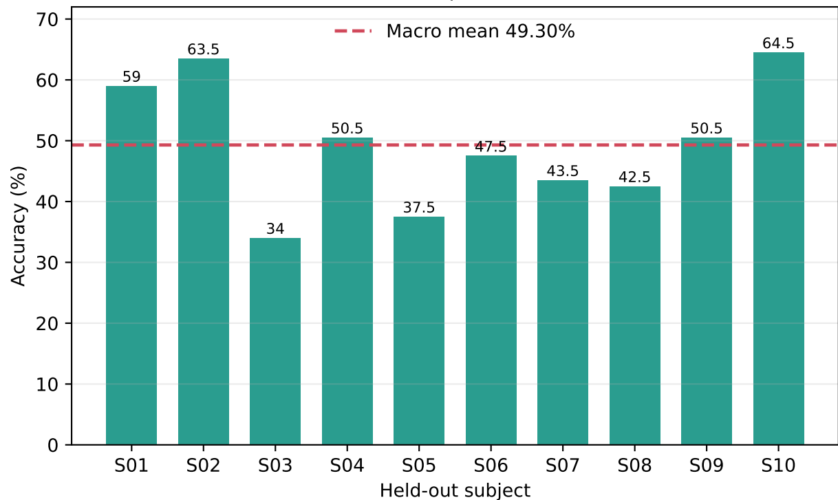
Top-5
