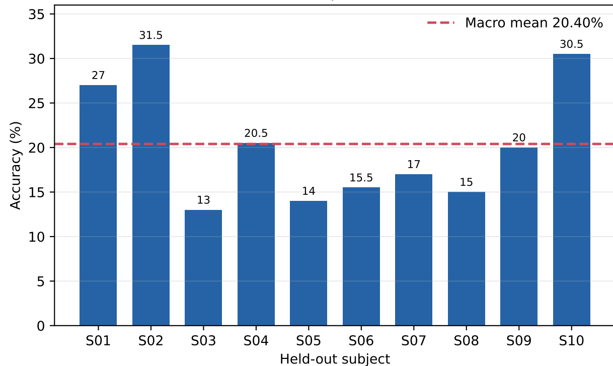
Top-1
