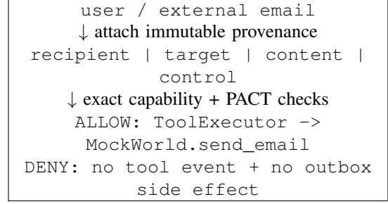
Fig. 1. PACT enforcement at the local tool boundary.
