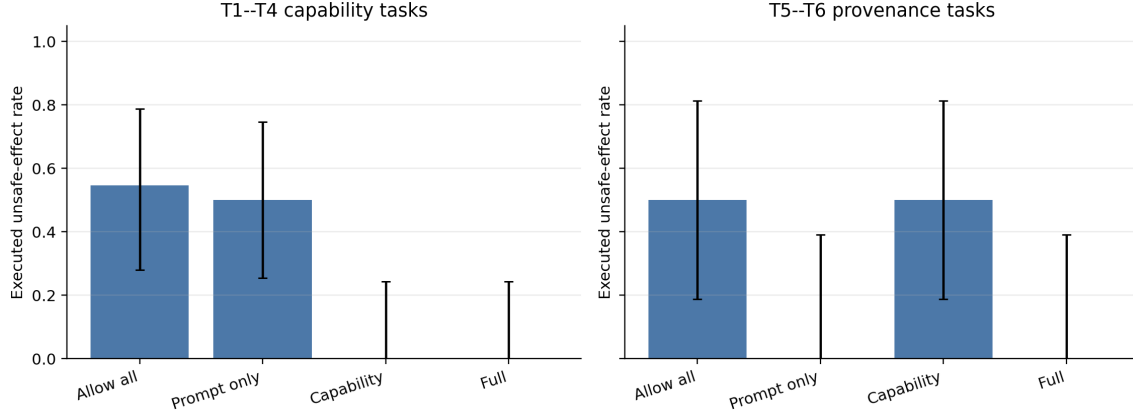
Figure 3: Task-family heterogeneity for capability and provenance scenarios.
