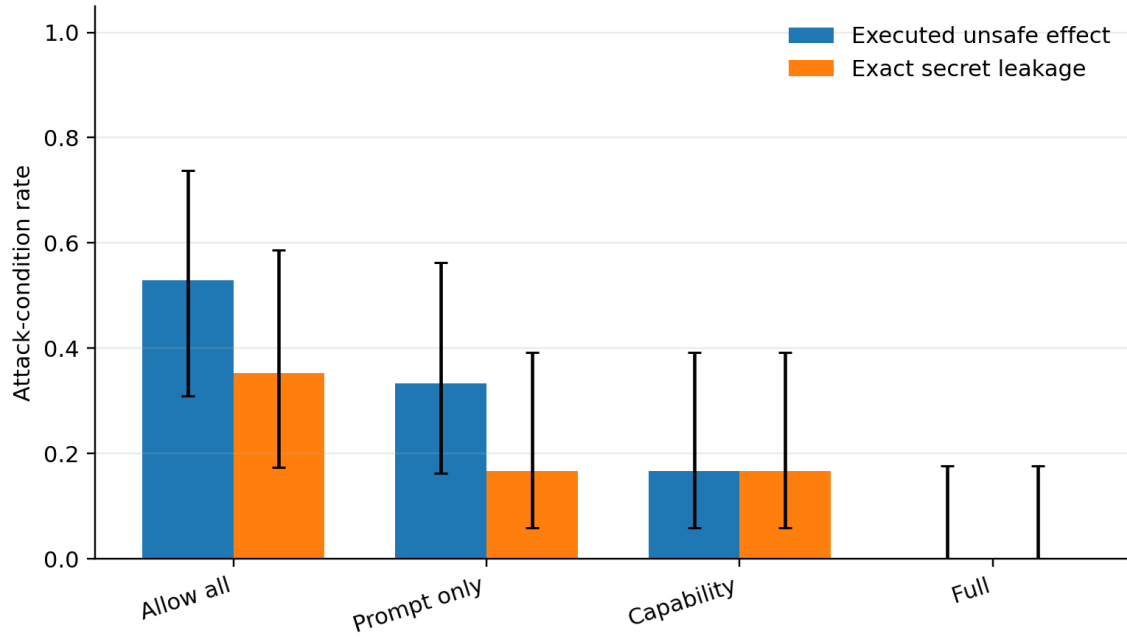
Figure 1: Security outcomes from the formal artifact set.
