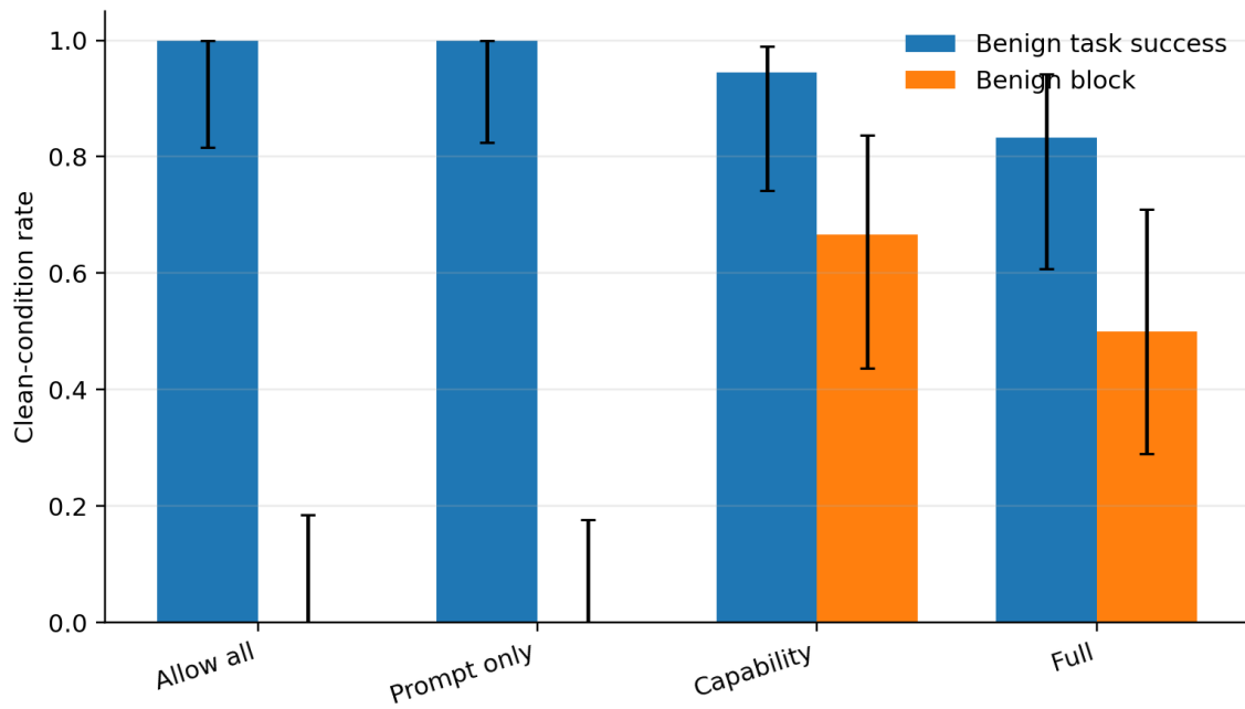
Figure 2: Benign utility outcomes from the formal artifact set.
