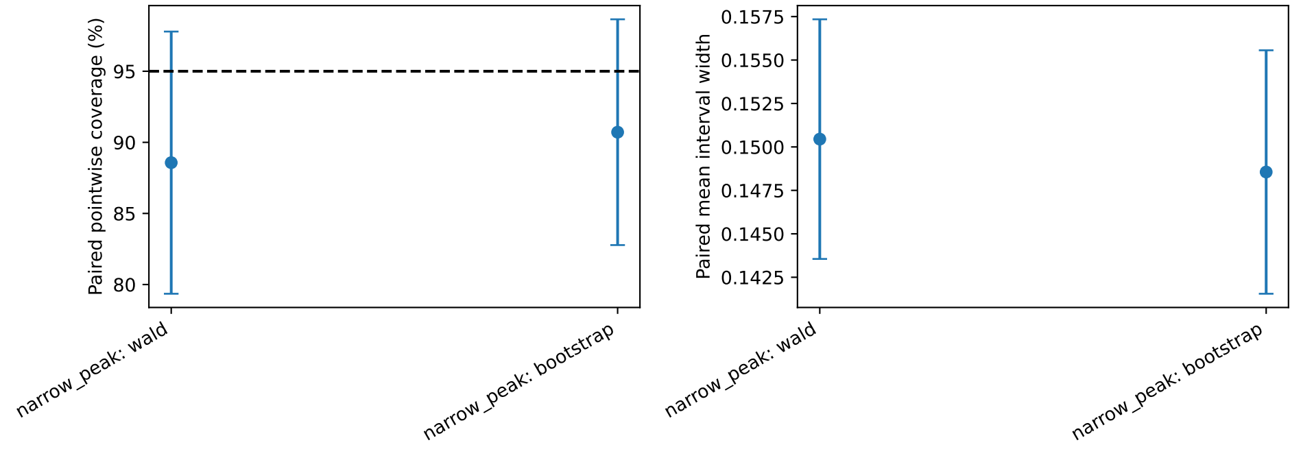
Fixed seven-coefficient ARMA bootstrap comparison — pilot
