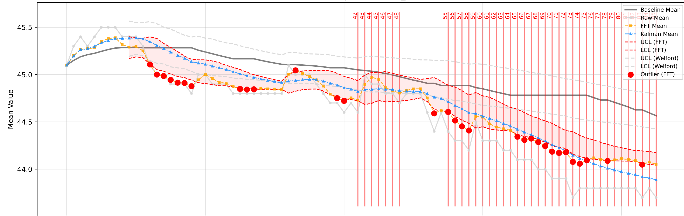
Target: VALUE (Individual X) | Group: ('LOT_01', 'P02M07C031P0')
