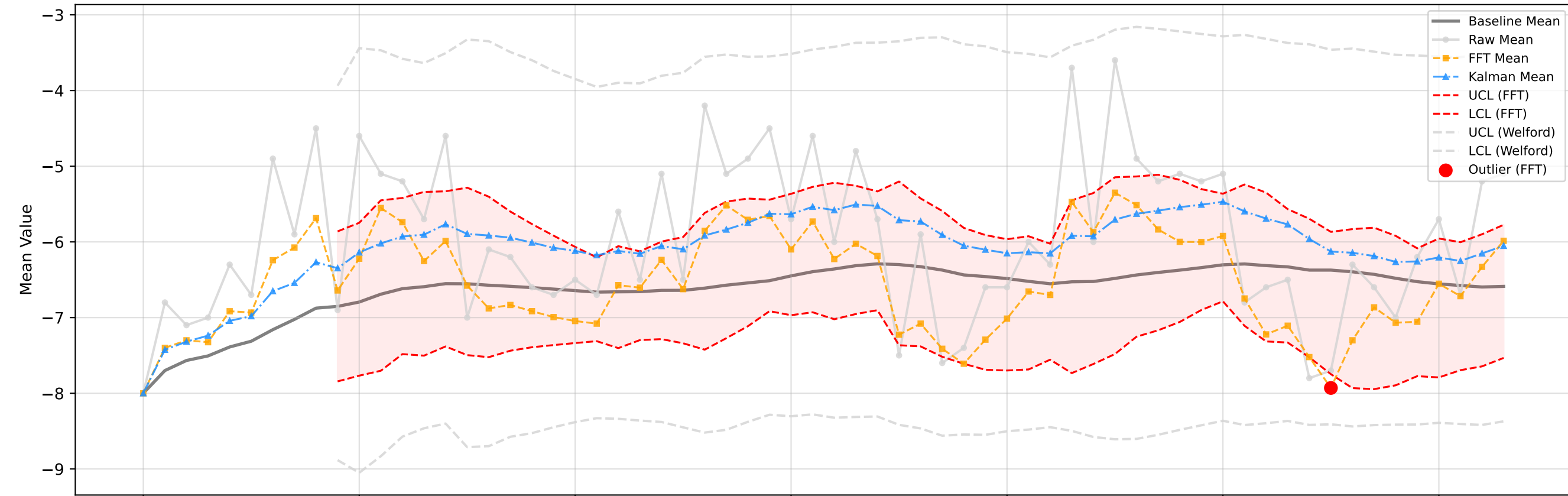
Target: VALUE (Individual X) | Group: ('LOT_02', 'P09M04C002P0')
