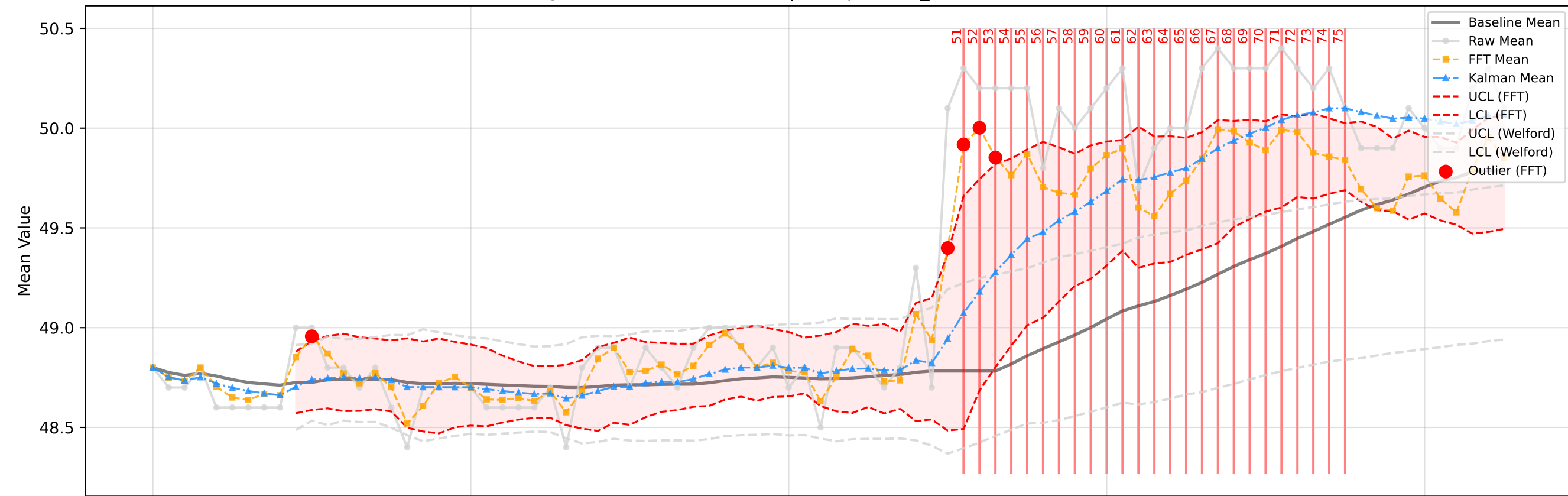
Target: VALUE (Individual X) | Group: ('LOT_01', 'P04M01C002P0')
