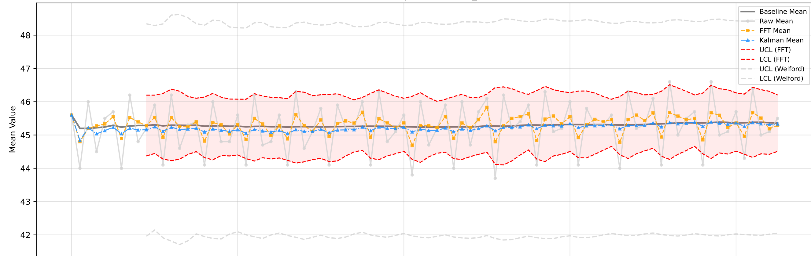
Target: VALUE (Individual X) | Group: ('LOT_01', 'P04M01C004P0')
