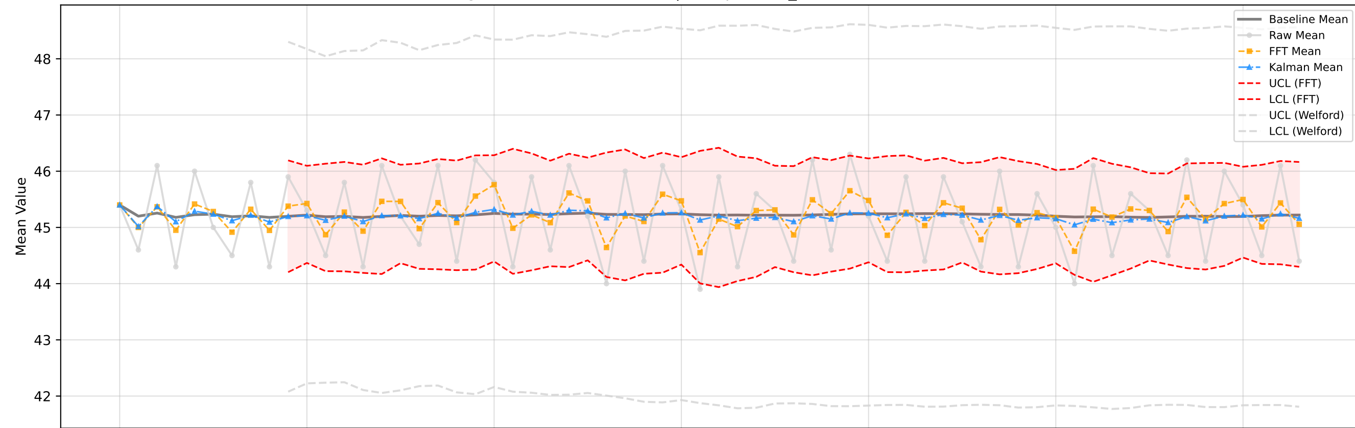
Target: VALUE (Individual X) | Group: ('LOT_02', 'P04M01C004P0')
