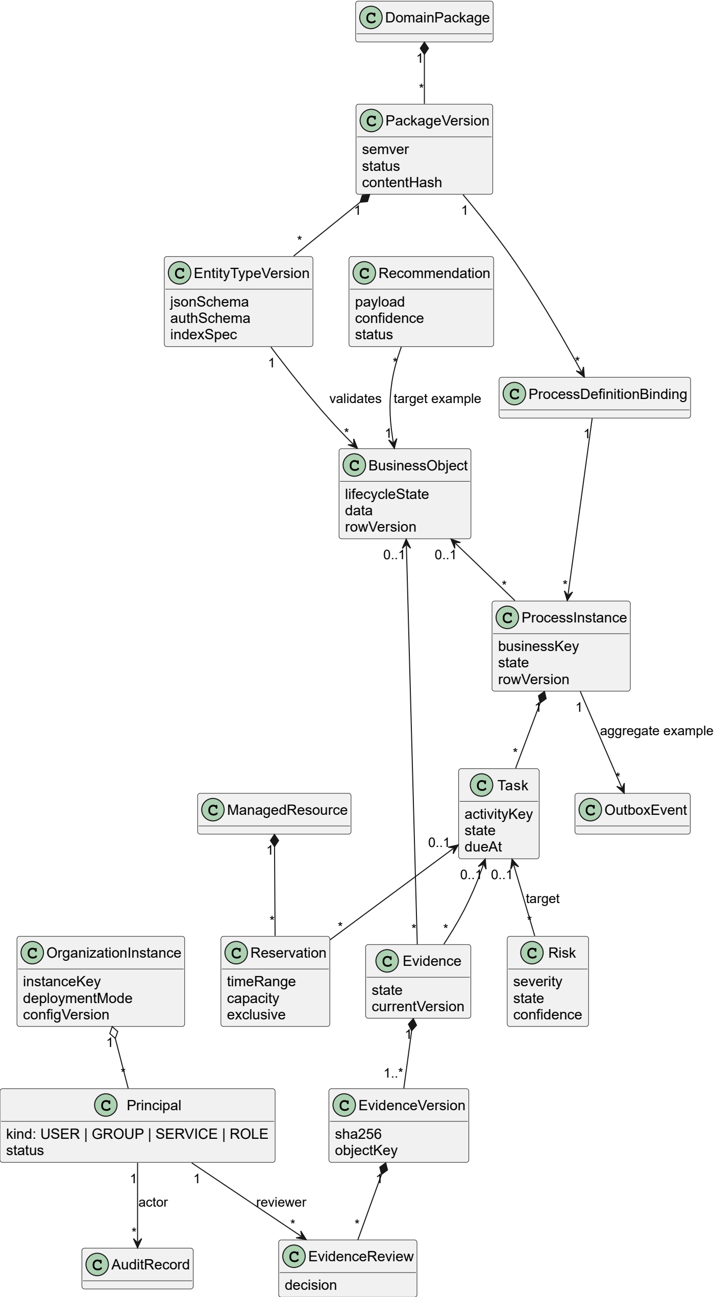
Innorder OCC - Domain Model
