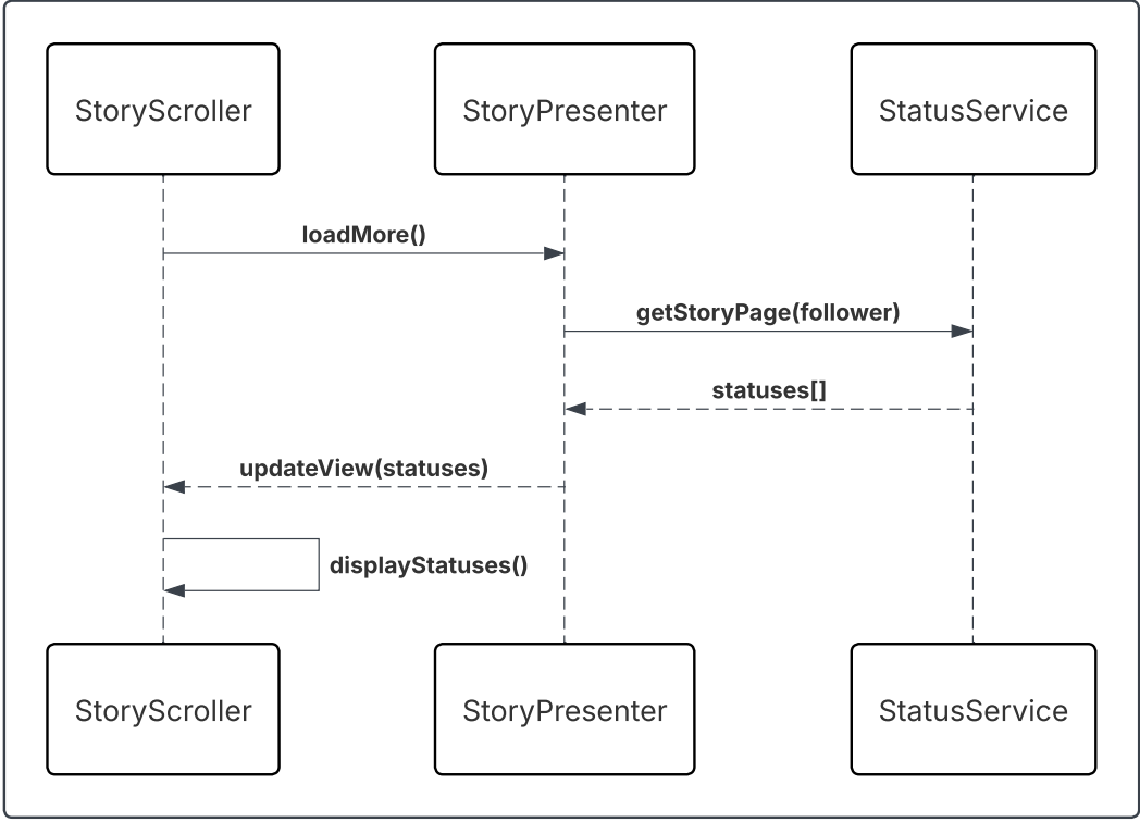
"Load More" Sequence Diagram
