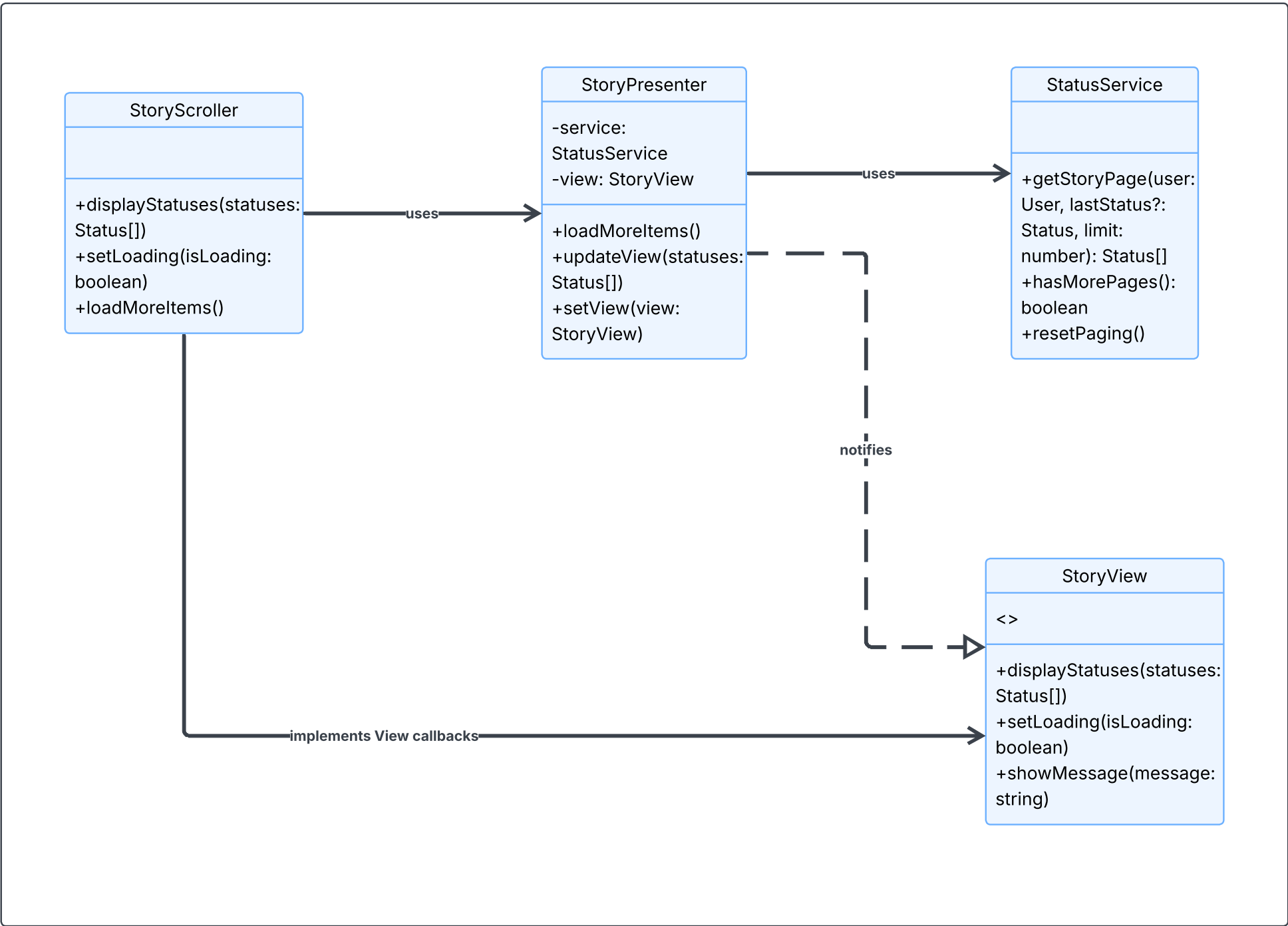
MVP Architecture Class Diagram
