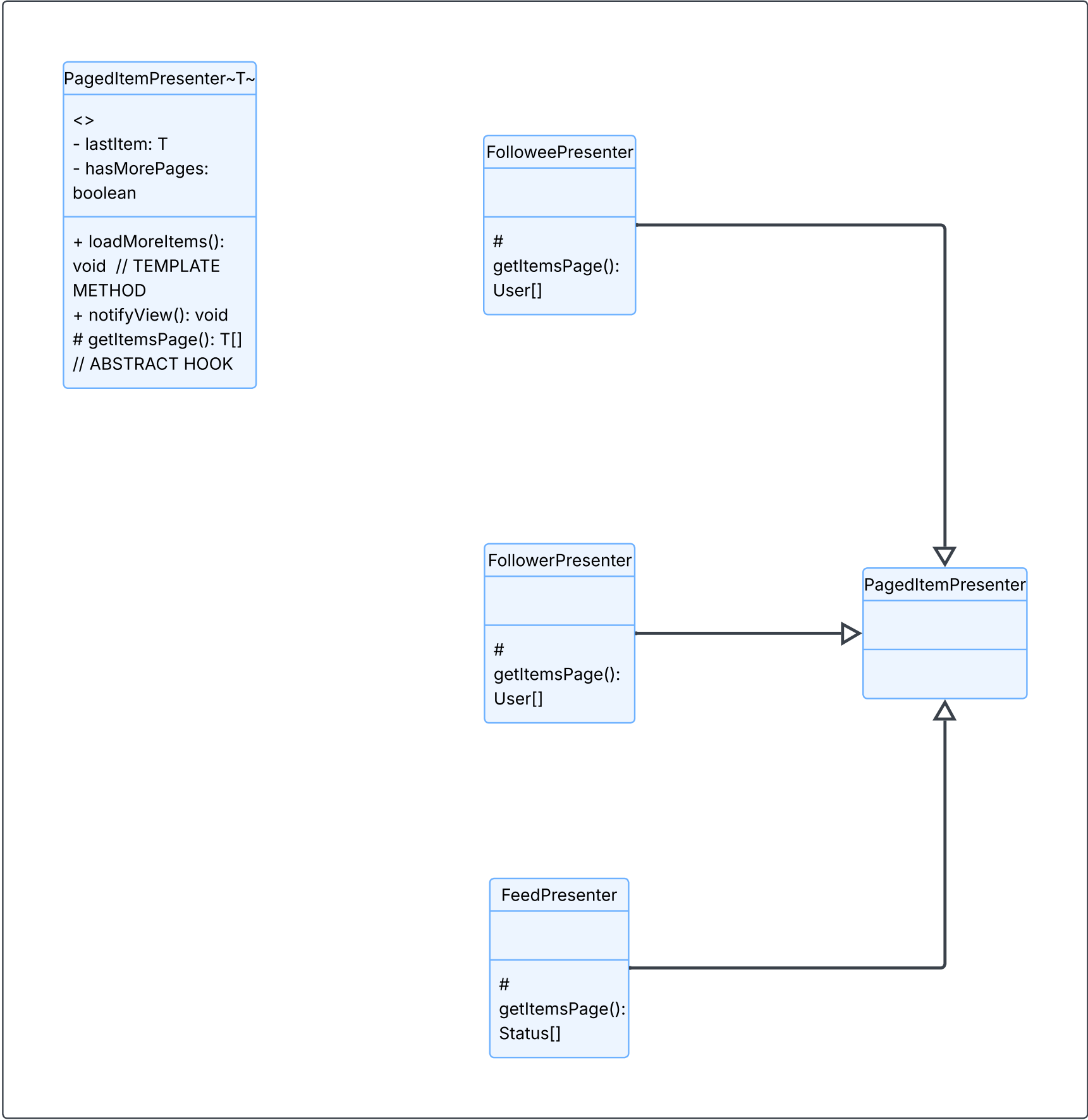
Template Method Pattern UML Diagram
