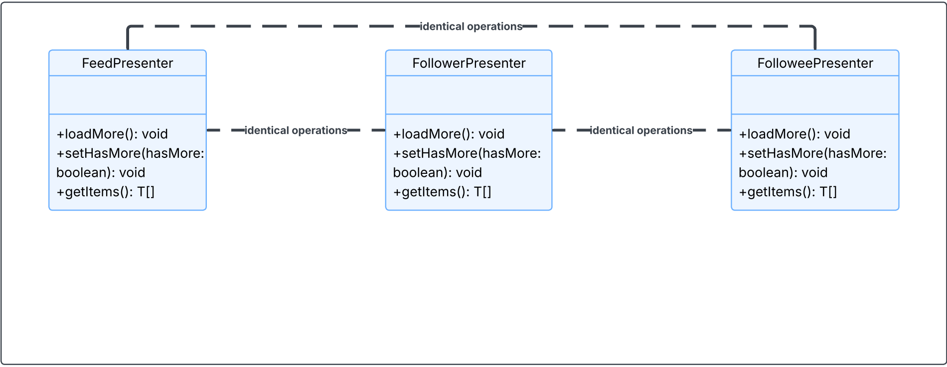
UML Class Diagram: Pre-Template Method
