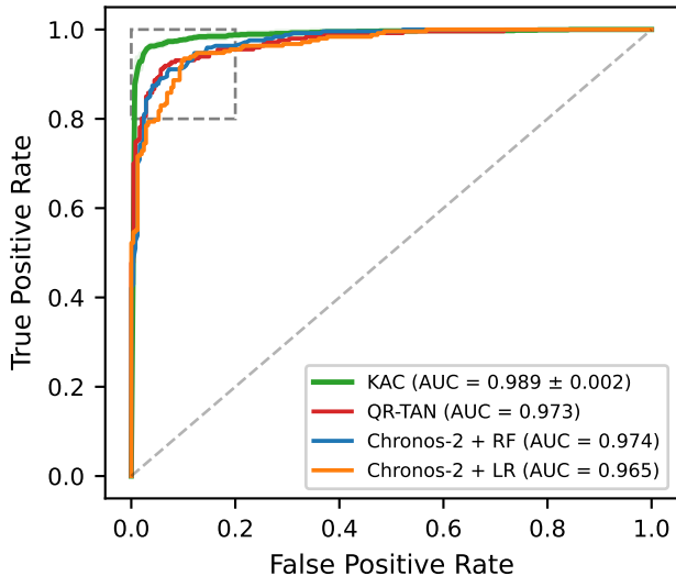
ROC Curve (Full)
