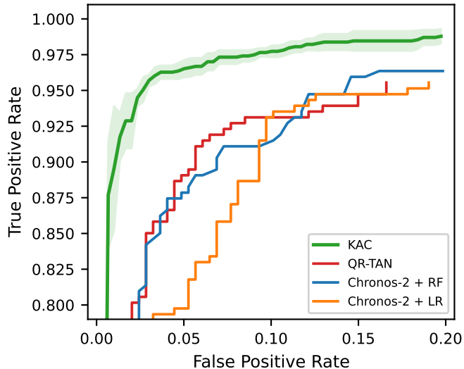
ROC Curve (Zoomed: FPR \leq 0.2 )
