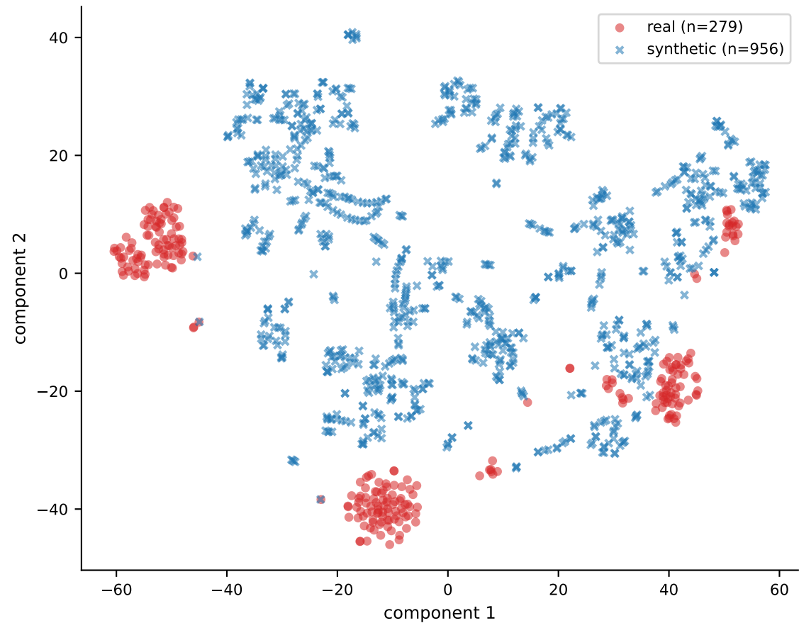
t-SNE (perplexity=30)
