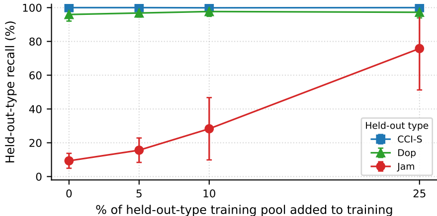
Calibration mini-sweep across three held-out anomaly types
