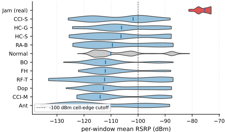
TelecomTS per-anomaly-type RSRP distributions (real Jamming highlighted)
