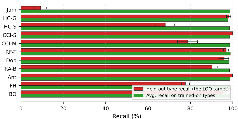
TelecomTS leave-one-anomaly-out audit (HGB on 240 KPI summaries; 10 seeds; 95% bootstrap CI on held-out recall)
