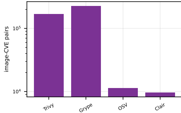
(b) Coverage
