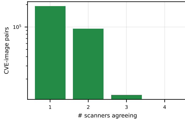
(c) Agreement
