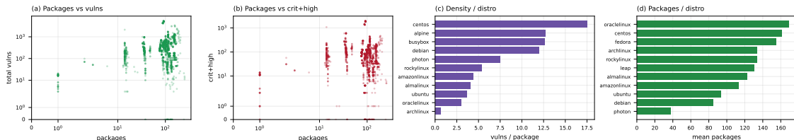
Figure 5. (a) packages vs. total; (b) packages vs. critical+high; (c) vulnerabilities per package by distribution; (d) packages per distribution.
