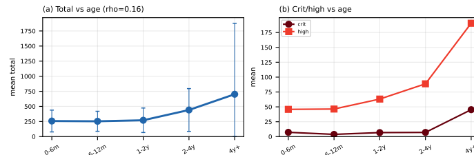
Figure 2. (a) mean total vulnerabilities by image age ( \pm 1 SD); (b) critical and high by age.
