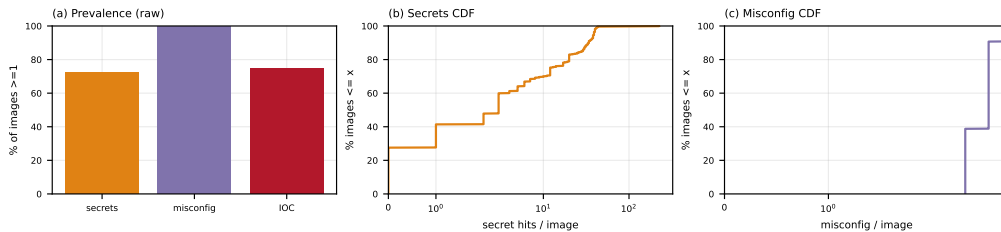
Figure 6. (a) raw detector prevalence; (b) secrets per image; (c) misconfigurations per image.
