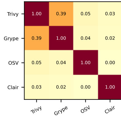
(a) Jaccard (CVE)
