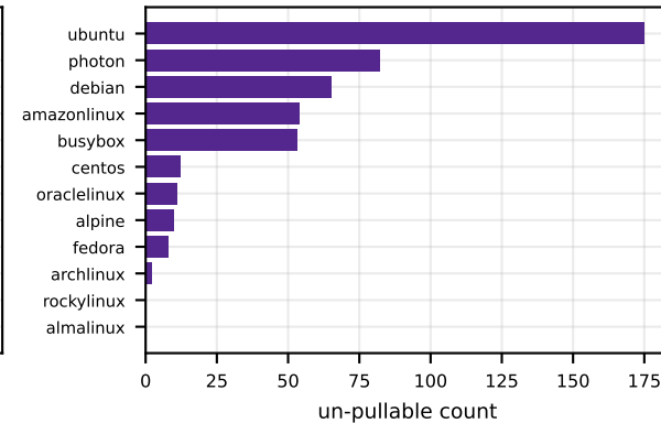
(c) Absolute
