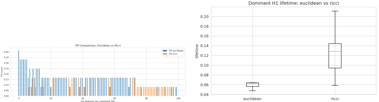
Figure 2: LUAD TIP and H_1 lifetime diagnostics comparing Euclidean and Ricci backends.
