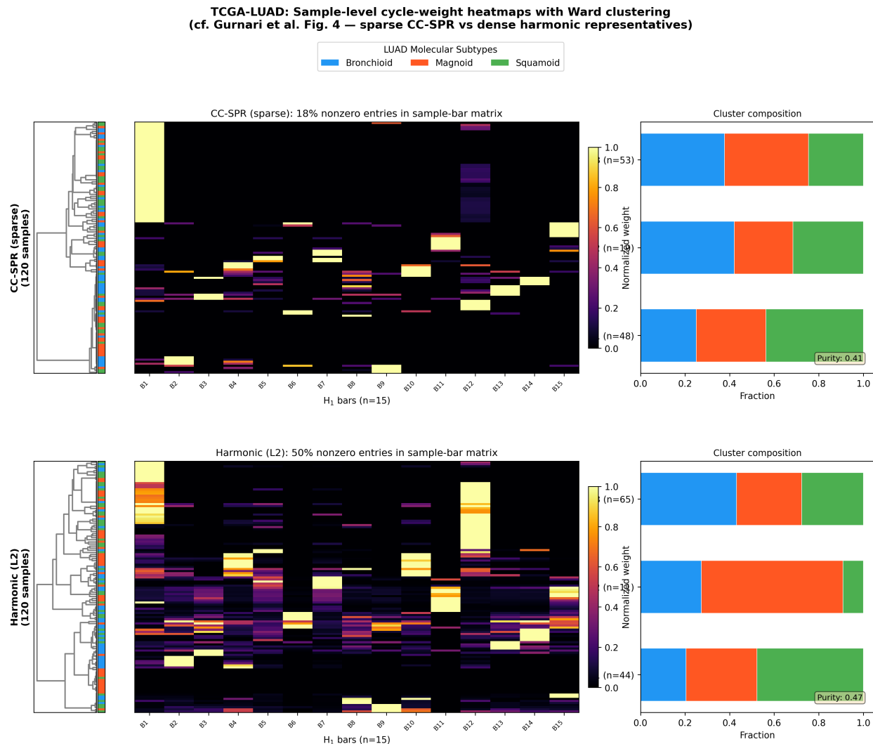
Figure 4: Sample-level cycle-weight heatmaps for LUAD (120 samples \times 15 H_1 bars). Top: CC-SPR—18% nonzero. Bottom: Harmonic—50% nonzero.
