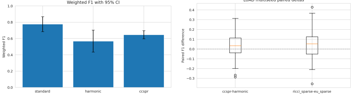
Figure 1: Left: LUAD benchmark showing the predictive gap between standard baseline and topology-derived models. Right: Paired multiseed deltas across 18 splits.
