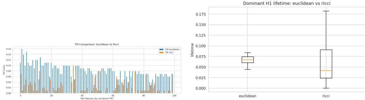
Figure 3: GSE161711 topological diagnostics. Left: TIP comparison. Right: H_1 lifetime comparison.
