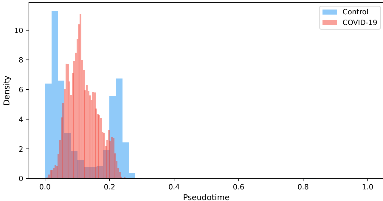
Pseudotime distribution by condition
