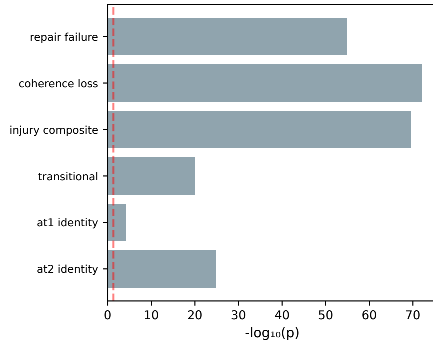
(b) Condition separation (MW)
