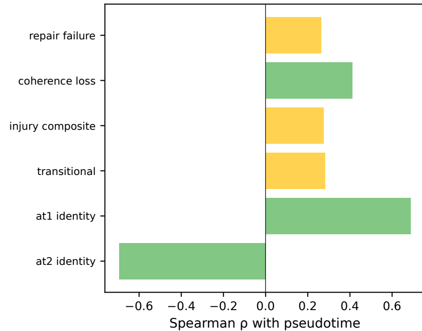
(a) Pseudotime correlation
