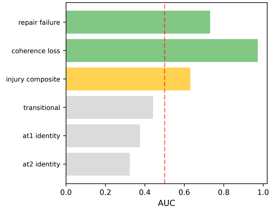
(c) Transitional cell detection AUC
