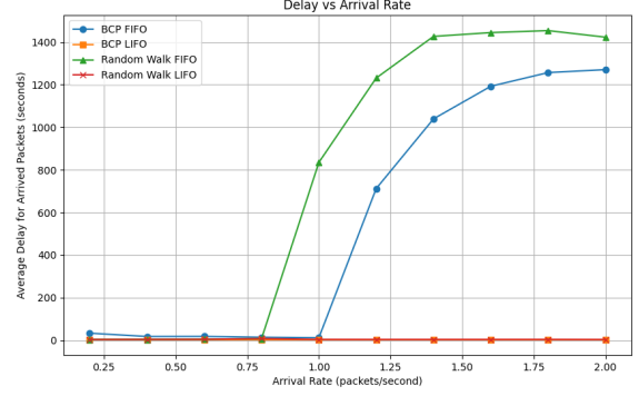
Figure 3: Average delay for successfully delivered packets versus arrival rate.
